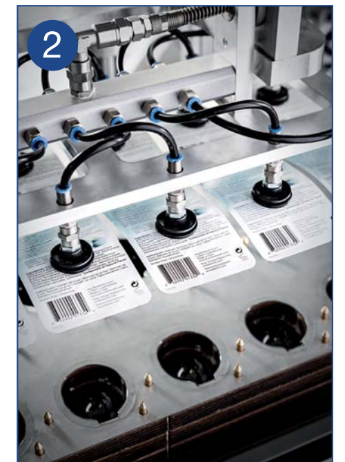
Automatic card feeder
